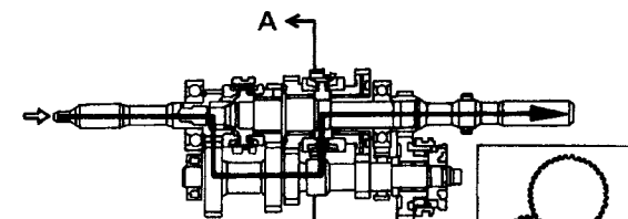
Reverse Idler Gear
