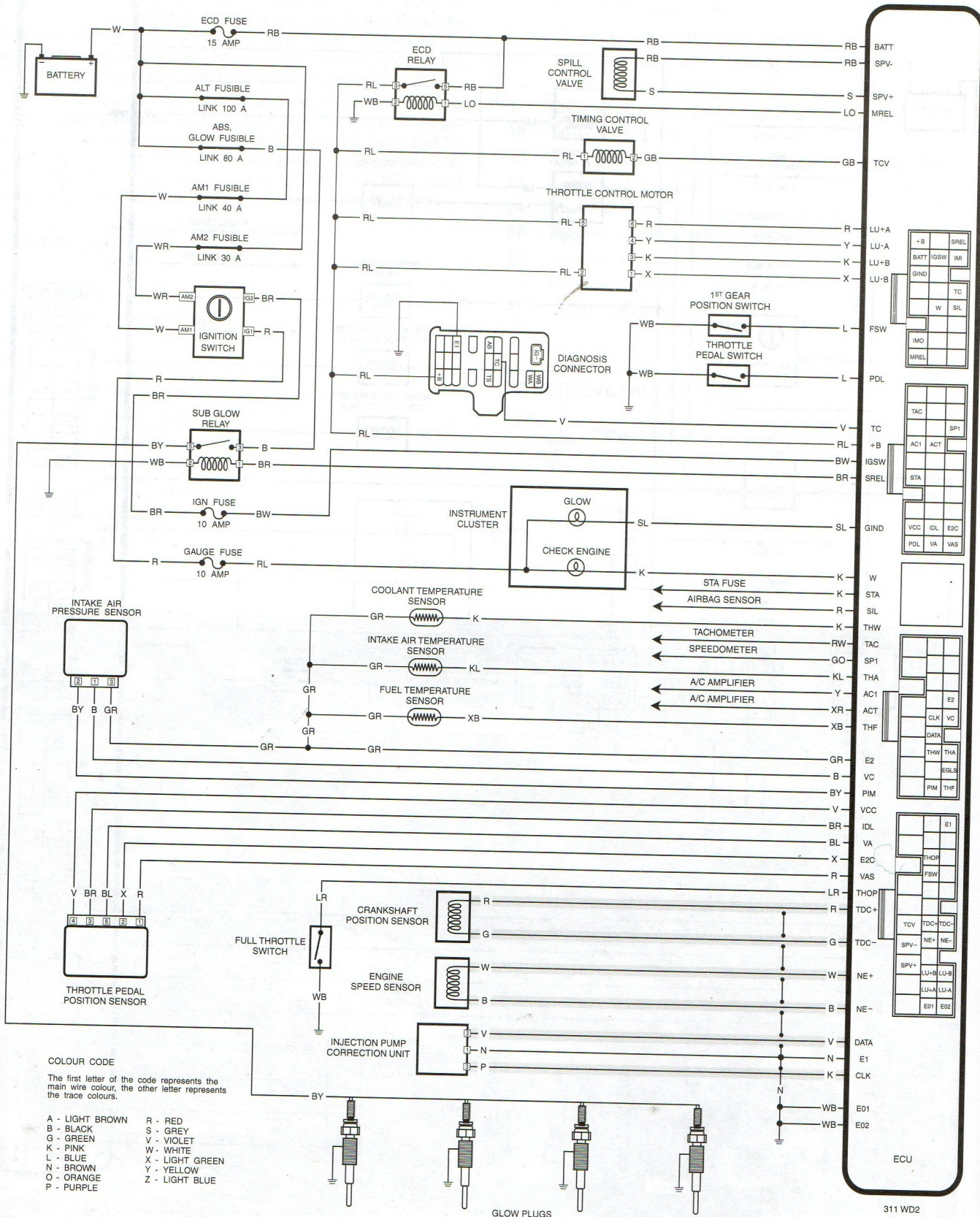
Fuel and engine management system. Late models.
