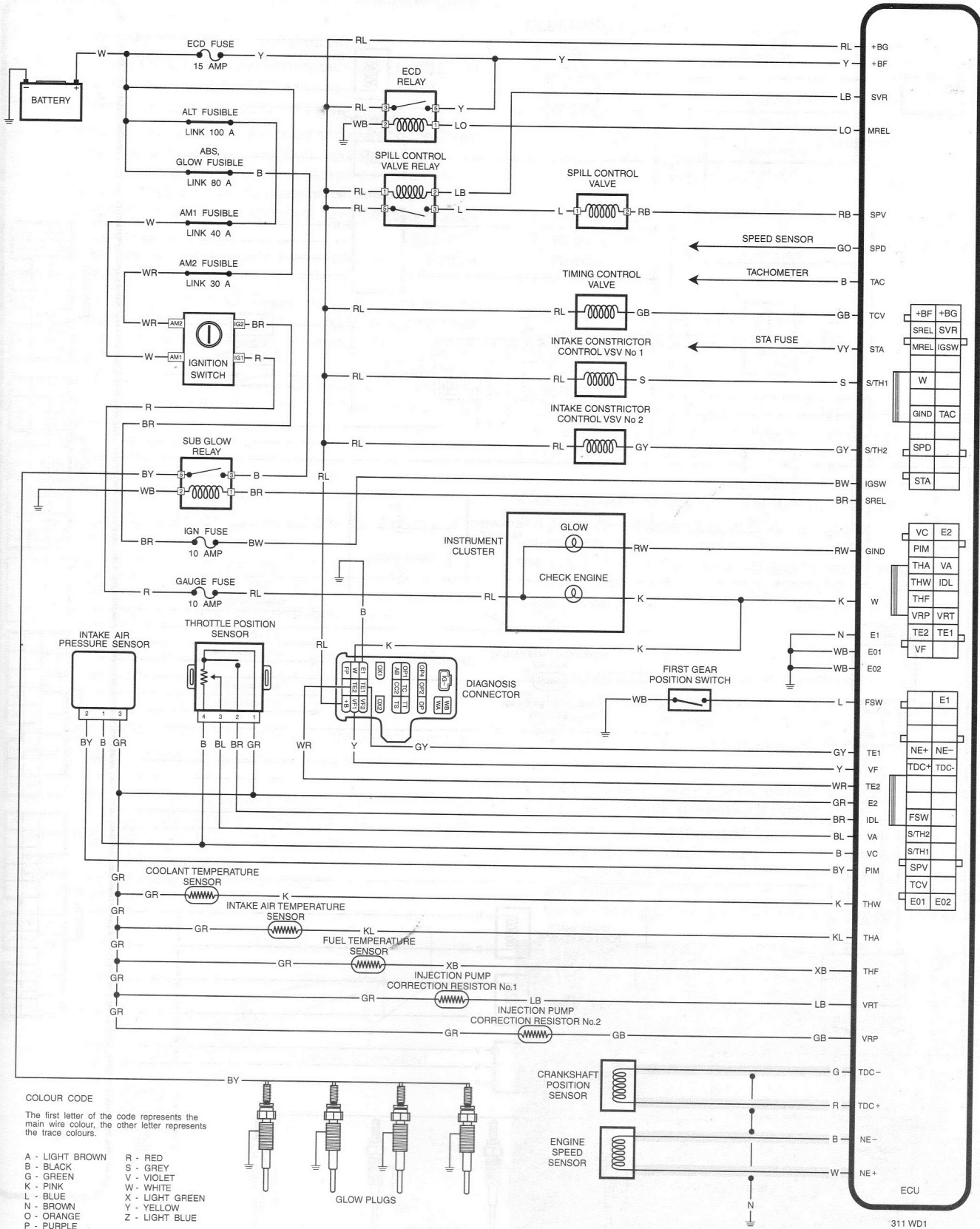
Fuel and engine management system. Early models.
